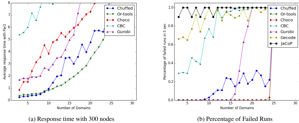
Figure 3: Solvers Comparison
