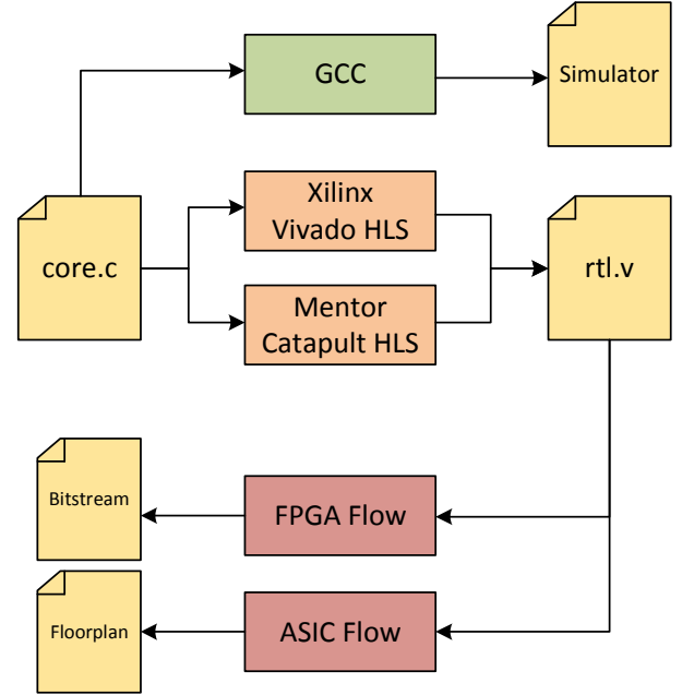
Fig. 1. Description of the design flow used for the Comet core. The flow only uses C++ source files as input and uses HLS tools to generate an RTL description of the core. This HDL file can be mapped into FPGA or ASIC. The same source files can be compiled to generate a fast, cycle and bit-accurate simulator of the core.
