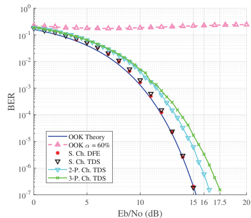
Fig. 5. Demodulation performance BER scaling according to SNR for the considered techniques with \alpha = 60\% .
