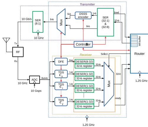
Fig. 3. Enhanced digital-domain transceiver architecture.
