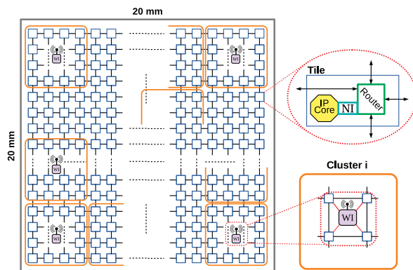
Fig. 1. Wireless interface distribution among a clustered WiNoC hybrid topology with N clusters of M cores.
