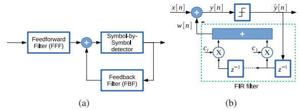
Fig. 2. (a) General DFE structure, (b) Adopted DFE.
