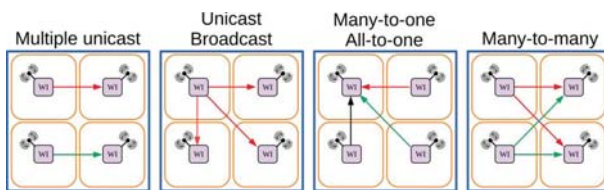
Fig. 4. Wireless communication patterns for a clustered WiNoC hybrid topology with N = 4 clusters.
