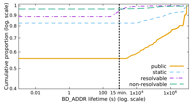
Figure 3: Empirical cumulative distribution function for lifetimes of device addresses.
