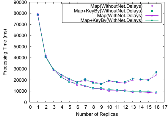
Figure 10: Effect of KeyBy on processing time.
