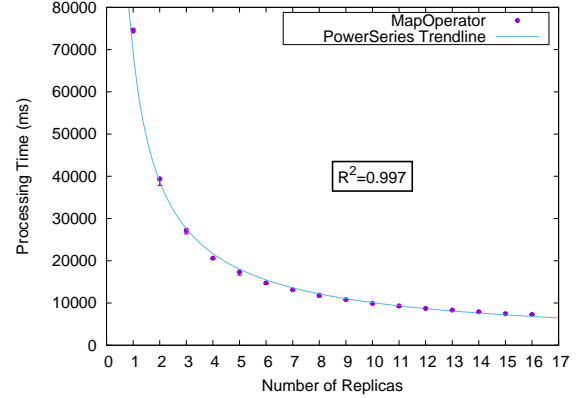
Figure 5: Effect of operator replication on processing time.
