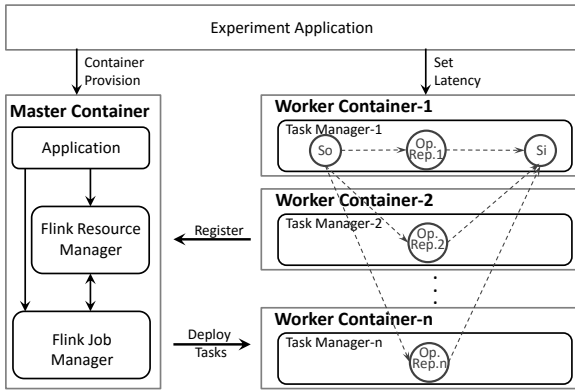
Figure 2: Experimental architecture.
