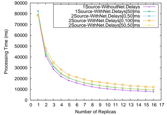
Figure 9: Effect of multiple sources on processing time.
