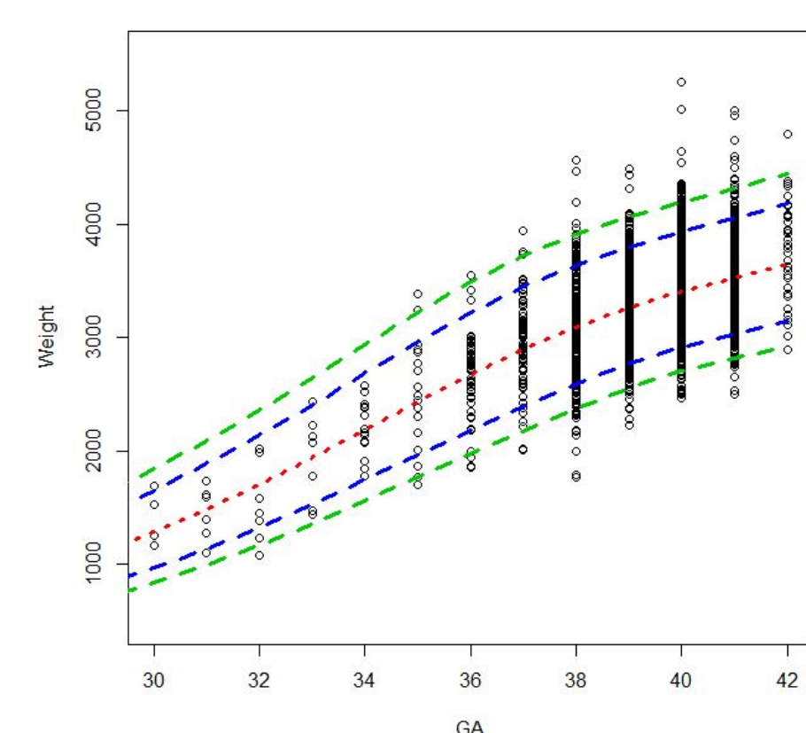
Figure 3: 3rd, 10th, 50th, 90th, 97th centile curves.
