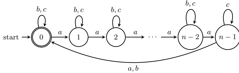
Fig. 3. The DFA A_n
