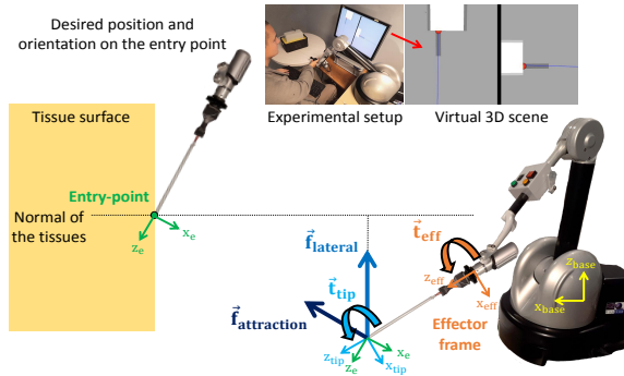
Figure 1: The five proposed haptic guide and the experimental setup of the preliminary user study. The blue arrows represent the needle-tip frame and forces and a torque expressed in the latter. FTip, TTip, FTTip and FTATip implement one or a combination of those forces and torque. The orange arrows represent the end-effector frame of the haptic device and a torque expressed in the latter, which is implemented by TEff.
