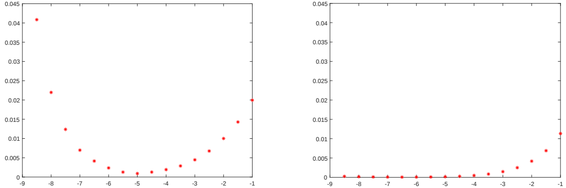
Figure 7: Curves \|u_{\varepsilon,h} - u\|_{H^1(\Omega)} (left) and \|u_{\varepsilon,h} - u\|_{H^1(\tilde{G})} (right) with respect to \log \varepsilon for h \approx 8.3 \times 10^{-3} .
