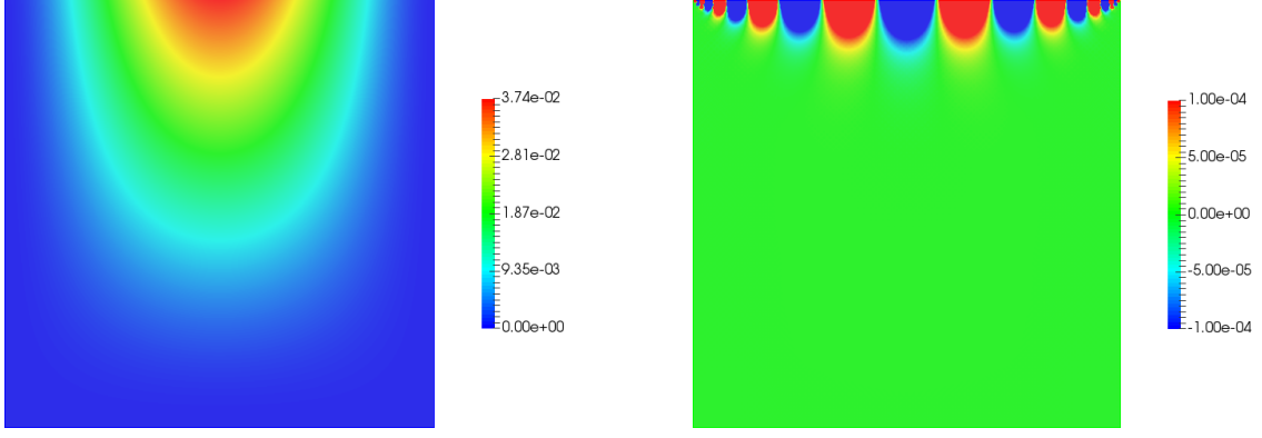
Figure 5: Exact solution u (left) and error u_{\varepsilon,h} - u (right) for \varepsilon = 10^{-8} , h \approx 7.1 \times 10^{-3} .
