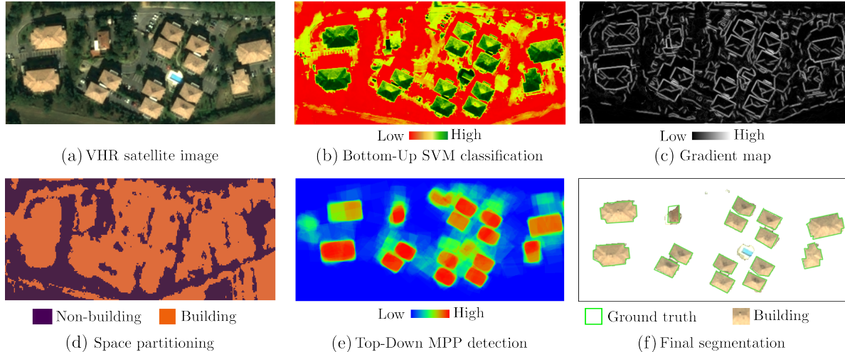
Fig. 1. Overview and sample result of our approach.
