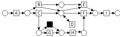
Fig. 11. A model with D in a self-loop
