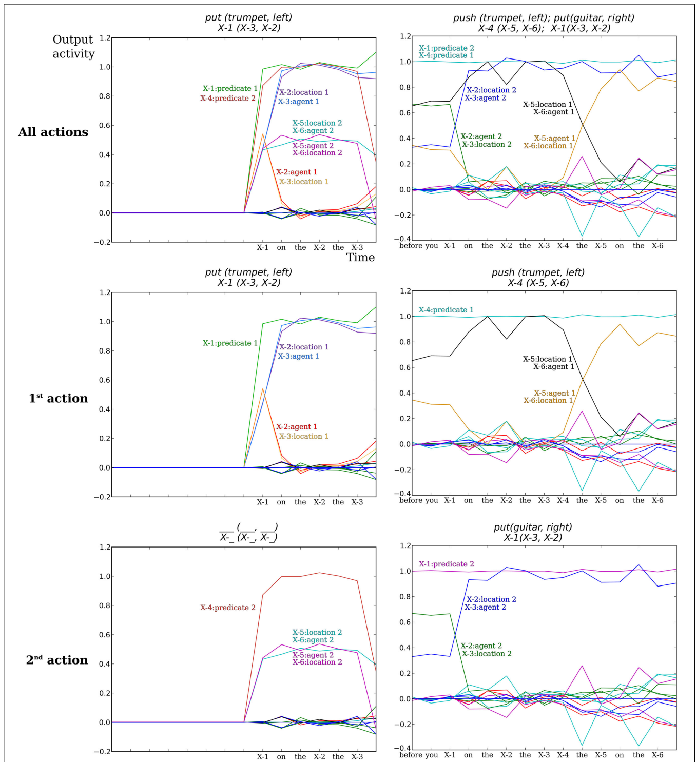
FIGURE 8 | Example of output activity of the comprehension neural model for the “Action Performing” task. Each colored line indicates the pseudo-probability for each semantic word to have a given role ( predicate, agent, location ) for each of the two specified actions. (Top row) Output activity for both actions. (Middle row) Output activity for the first action to perform. (Bottom row) Output activity for the second action to perform. (Left column) The input sentence was “put on the left the trumpet.” The model correctly determines that there is only one meaning-predicate put (trumpet,
