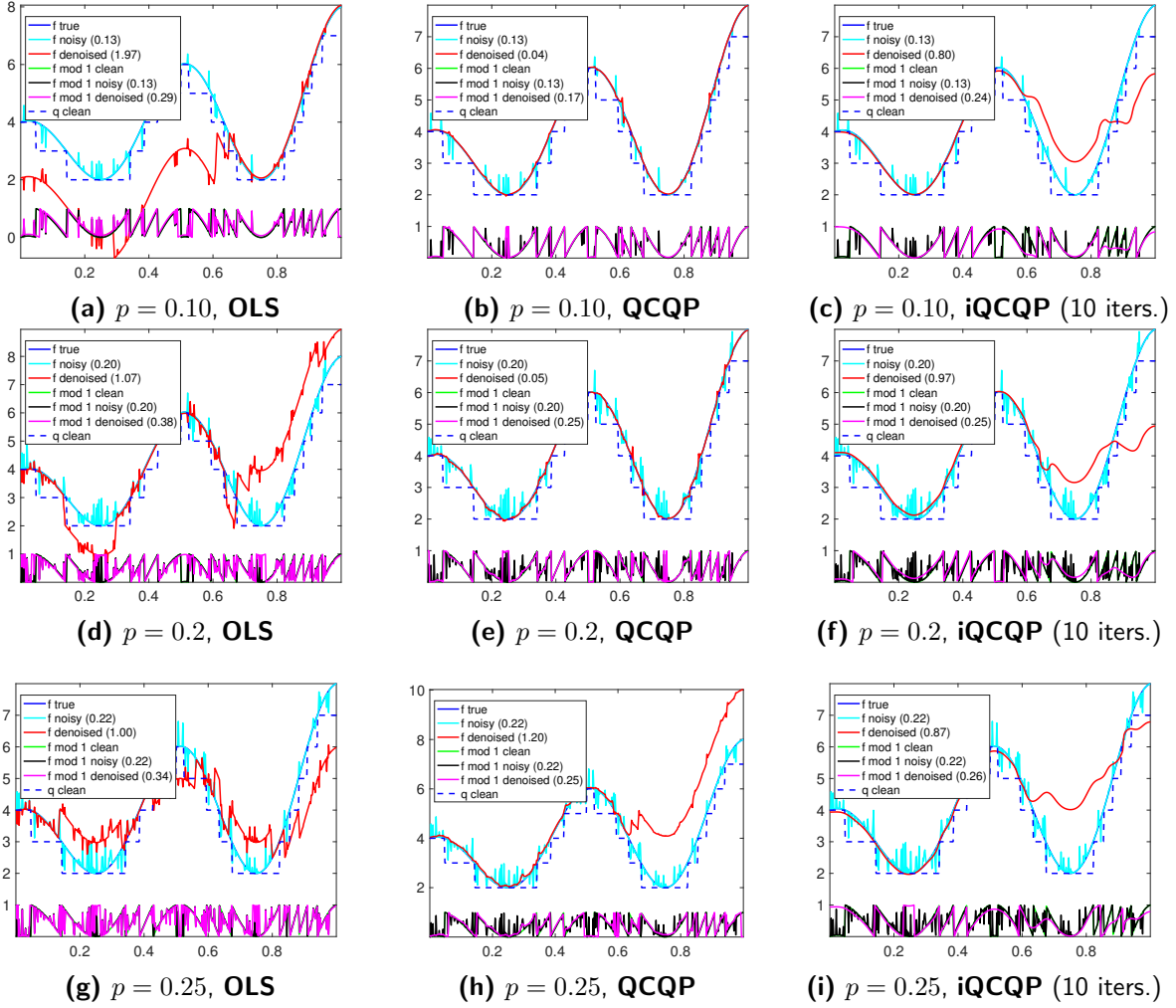
Figure 10: Denoised instances under the Bernoulli noise model, for OLS, QCQP (Algorithm 1) and iQCQP, as we increase the noise level \sigma . QCQP denotes Algorithm 1, for which the unwrapping stage is performed via OLS (4.23). We keep fixed the parameters n = 500 , k = 2 , \lambda = 1 .
