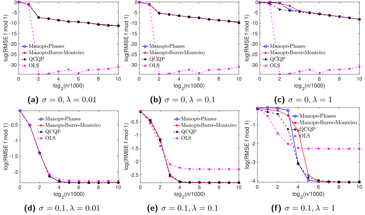
Figure 16: RMSE comparison for f \bmod 1 denoising, for the synthetic example f(x, y) = 6xe^{-x^2-y^2} , with k = 1 (Chebychev distance), while varying \sigma and \lambda . QCQP denotes Algorithm 1 where the unwrapping stage is performed via OLS (4.23).
