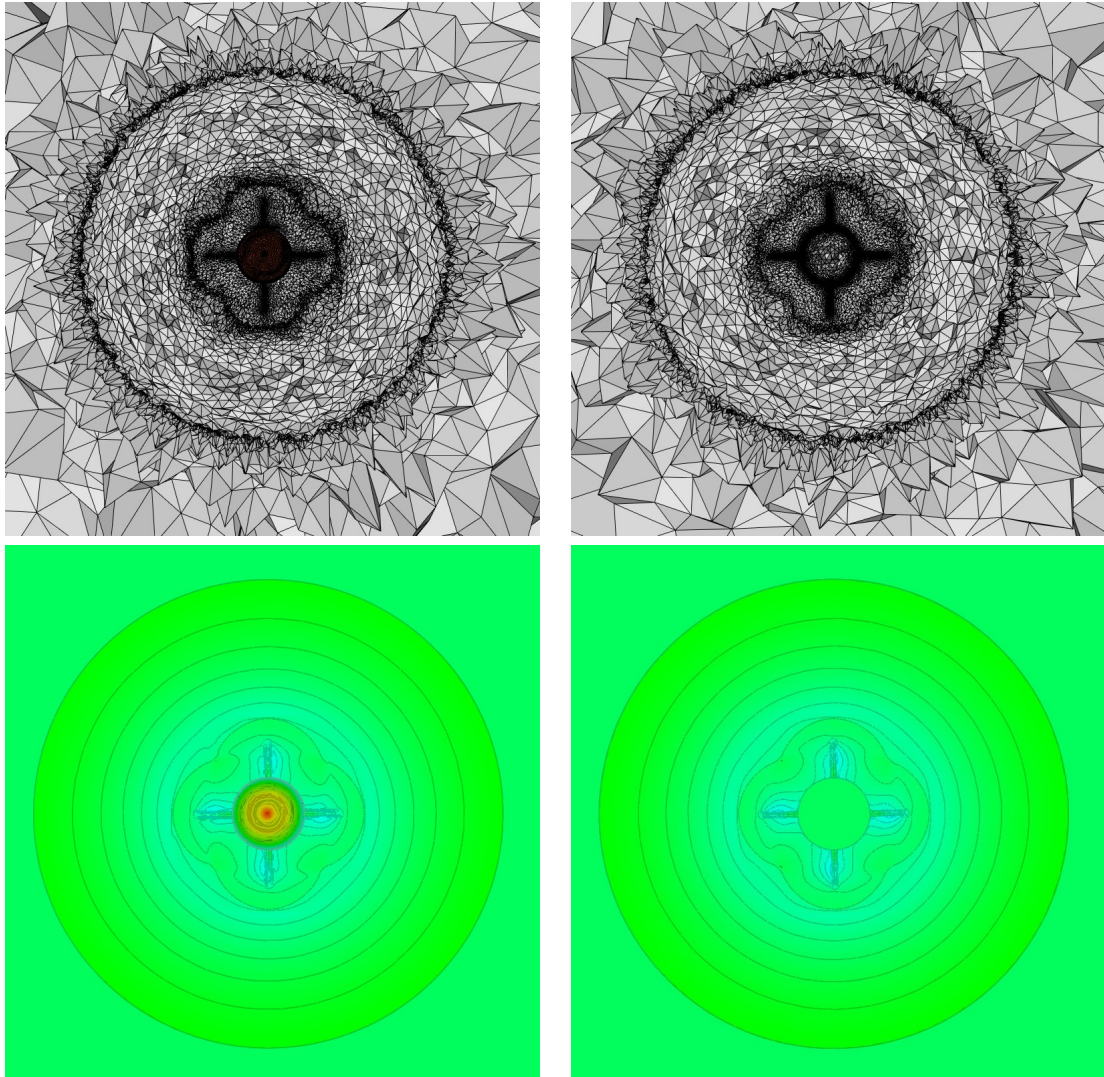
Figure 37: Supersonic flow around a notional missile. Left, adapted body-fitted case. Right, adapted embedded case. View along x = 0 axis. Top, the adapted meshes. Bottom, the associated solutions.
