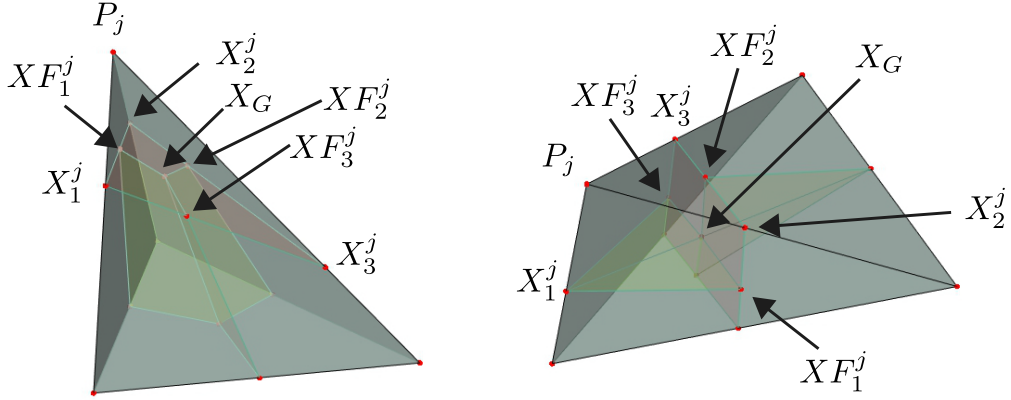
Figure 15: Two classic cases of cut-cell in 3D.
