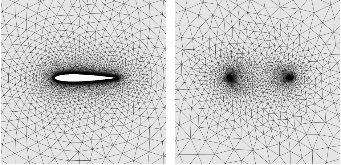
Figure 21: Body-fitted (left) and embedded (right) meshes used for the simulations of the flow around a NACA0012 airfoil.
