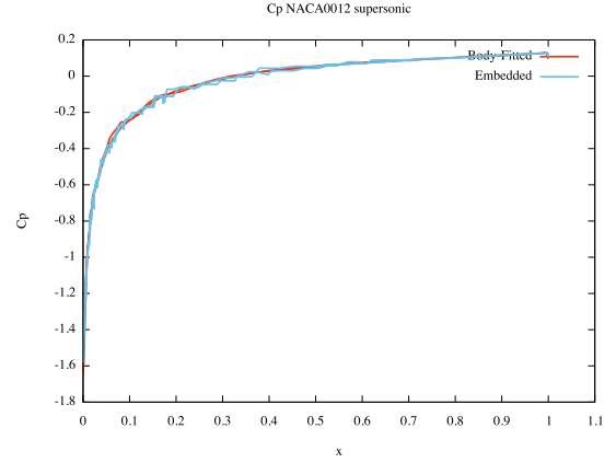
Figure 27: Computed C_p of a supersonic flow around a NACA0012 airfoil.
