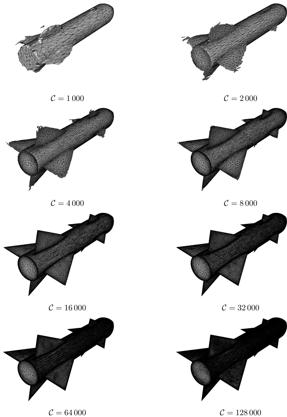
Figure 38: Evolution of the detection of the embedded geometry by the CFD solver all along the mesh adaptation process. Each of the 8 cases shows the result obtained at the last iteration of the adaptation process for a given complexity.
