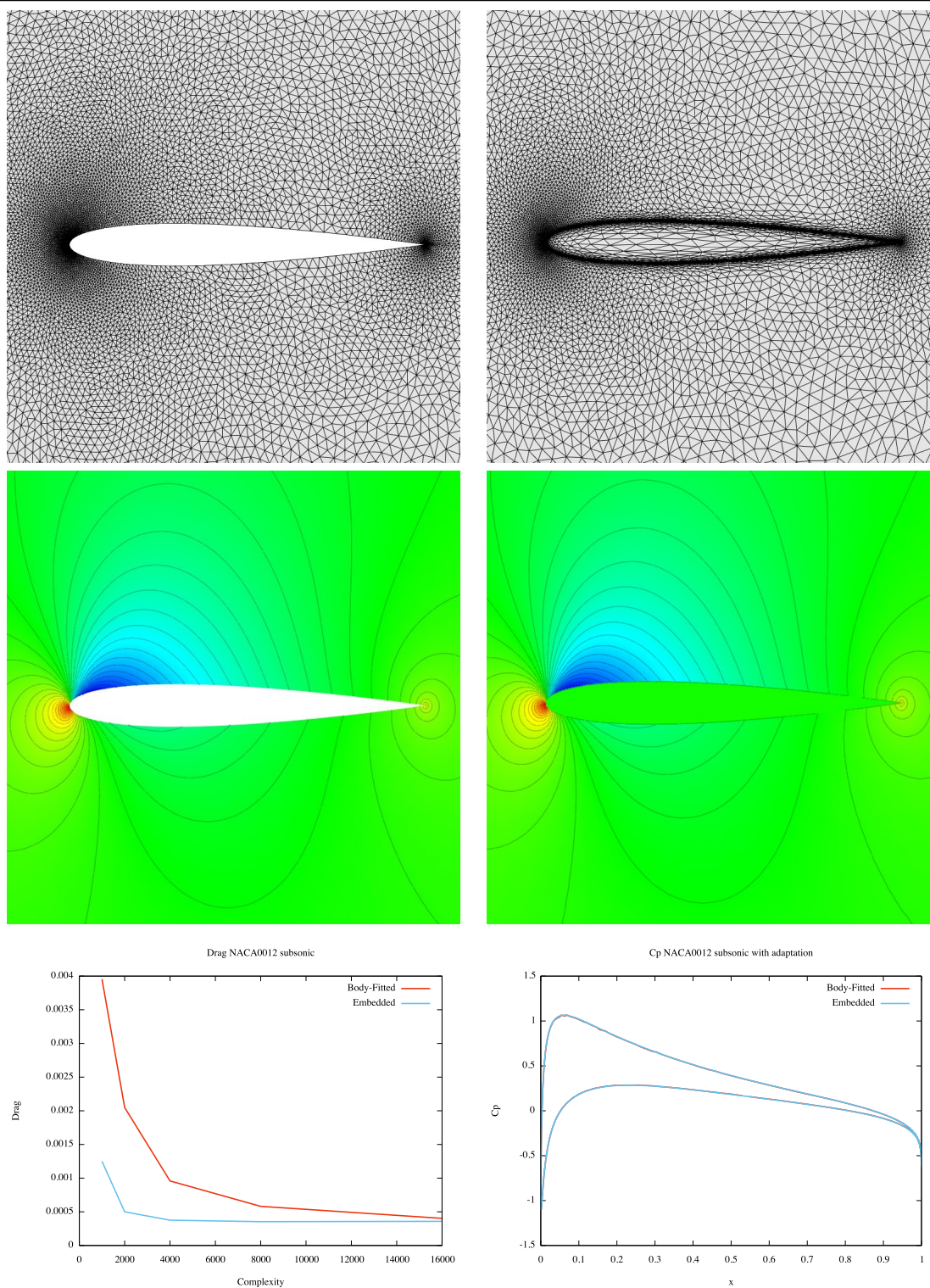
Figure 33: Subsonic flow around NACA0012 airfoils. Left, the adapted body-fitted case. Right, the adapted embedded case. Top, the adapted meshes obtained at the last complexity. Middle, the associated solutions density fields. Bottom, the evolution of the drag all along the adaptation process (left) and the C_p curves at the last complexity (right).
