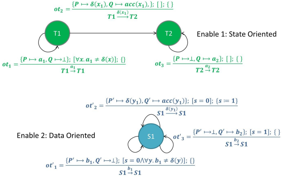
Figure 3: The two open automata
