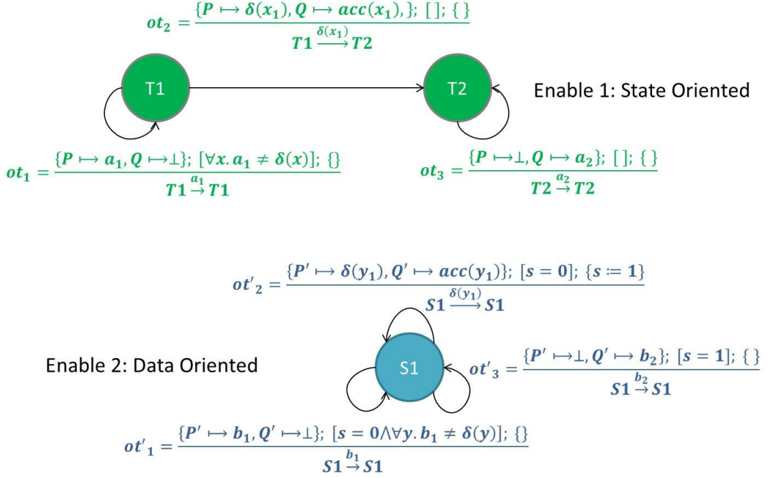
Figure 4: The two open automata
