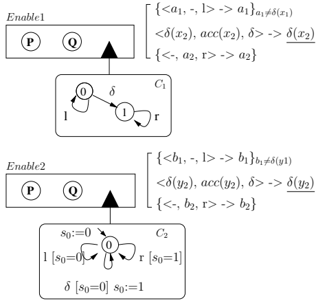
Figure 1: Two pNet encodings for Enable
