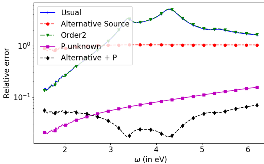
Figure 9: Relative L^2 error versus the pulsation \omega for the interior of the silicon square
