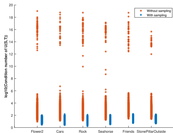
Fig. 9: Efficiency of the sampling and effect on the condition number of the matrix \mathbf{U}_k(S, T) . We show for each dataset, for all super-rays the log base 10 of the condition number without (red) and with (blue) sampling.
