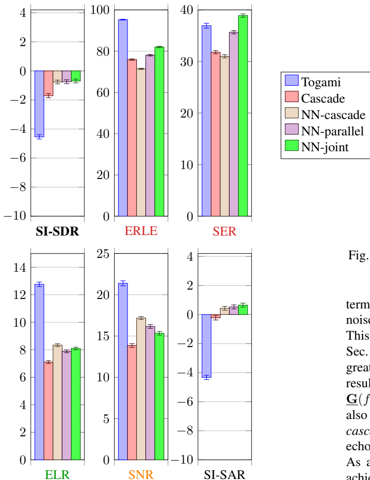
Fig. 10: Average results (in dB) in time-invariant conditions
