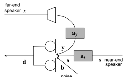
Fig. 1: Acoustic echo, reverberation and noise problem.
