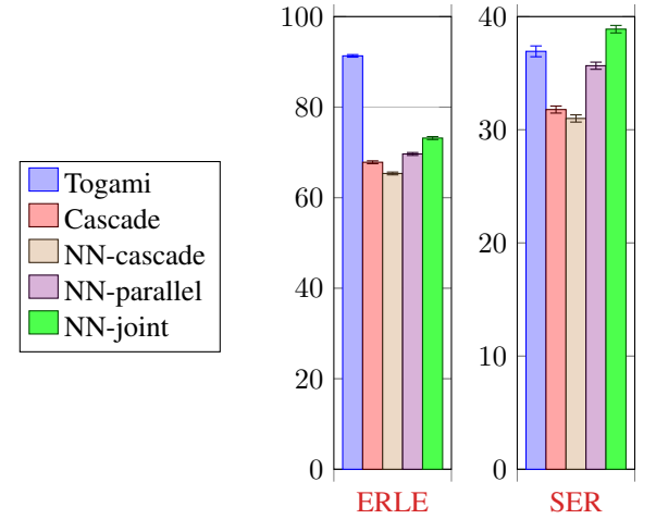
Fig. 13: Results (in dB) during double-talk in time-invariant conditions.
