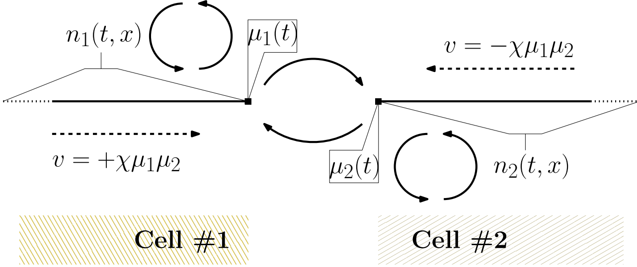
FIGURE 1. Cartoon of the model (2)-(3)-(4): the molecular content in the bulk experiences diffusion and transport at speed v = \pm \chi \mu_1 \mu_2 , where \mu_i can be seen as the fraction of activated molecules attached to the cell boundary. The dialog between the two cells arises as they secrete some communication signal (a pheromone) at a rate proportional to \mu_i , enhancing further the transport of molecular content in the opposite cell. Details are given in Section 2.
