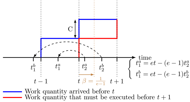
Figure 4: (BKP) with integer speed decision times ( t \in \mathbb{N} ) and Case 1 ( t_2 < t + 1 ). Let t_2^i \in (t, t + 1] with i \in \{a, b\} to illustrate the two sub-cases. Before t + \beta (sub-case i = a ), no jobs are taken into account in the speed computation, so S_{\max}^{(\text{BKP})} = 0 . After this threshold (sub-case i = b ), S_{\max}^{(\text{BKP})} can be non null because we take potentially into account the job arriving at t - 1 and ending at t . This job is at worst of size C . The two black arrows illustrate the position of t_1^i with respect to that of t_2^i .
