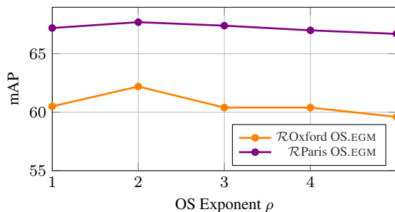
Fig. 9 mAP on \mathcal{R}_{\text{Oxford}} and \mathcal{R}_{\text{Paris}} versus saliency exponent \rho in OS.EGM.
