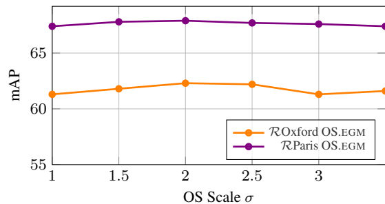
Fig. 10 mAP on \mathcal{R}_{\text{Oxford}} and \mathcal{R}_{\text{Paris}} versus EGM scale parameter \sigma in OS.EGM.
