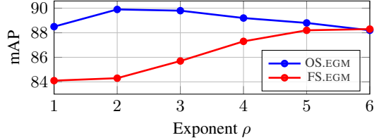
Figure 5. mAP on Oxford5k versus saliency exponent \rho for FS.EGM and OS.EGM.
