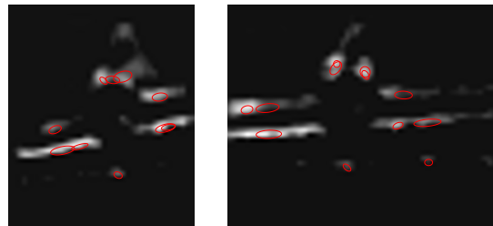
Figure 4. Feature maps from one channel for two different views of a building in the \mathcal{ROxf} dataset. Ellipses are fitted to the local features detected by MSER.
