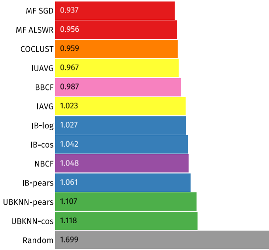
(a) ML-100K
