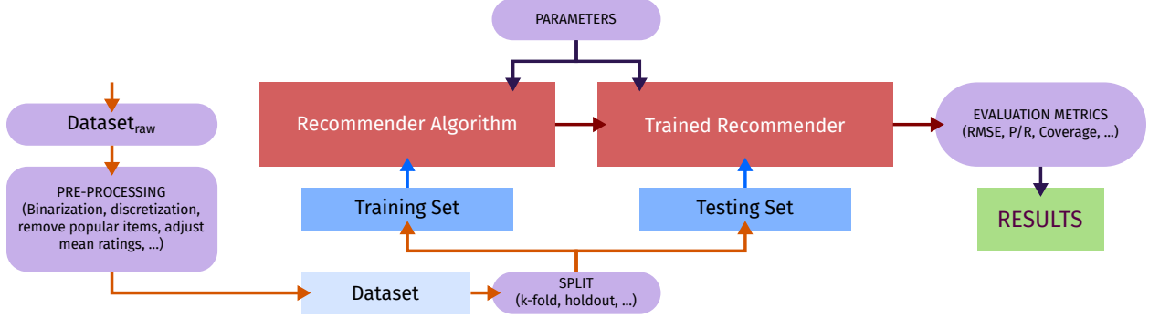
Figure 7: Offline evaluation of a recommender algorithm. Rounded purple boxes highlight the different elements where user choices may impact the final results.
