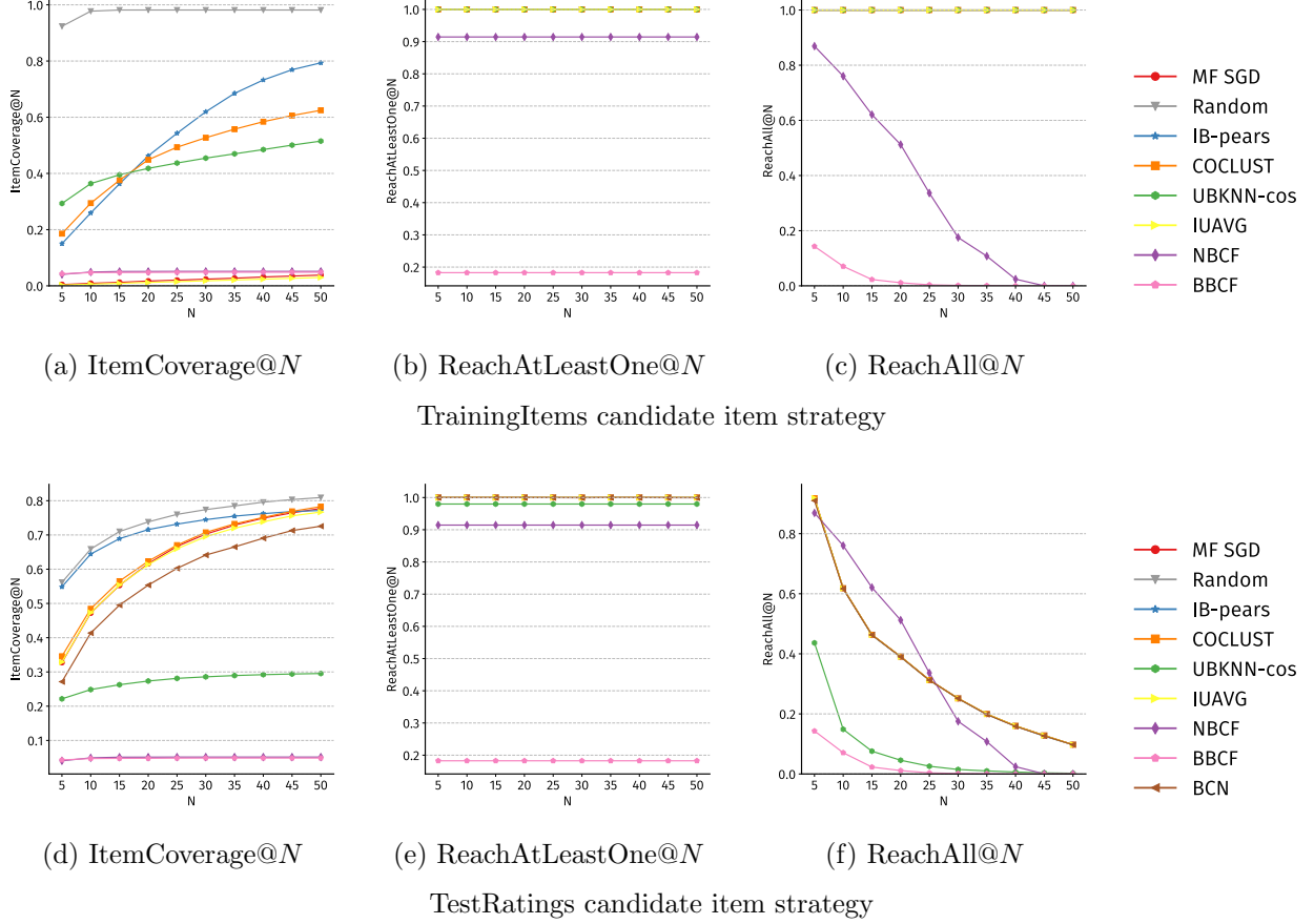
Figure 13: Coverage with the ML-100K dataset and N recommendations provided.
