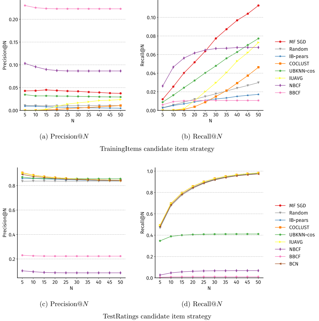
Figure 12: Precision / recall with the ML-100K dataset and N recommendations provided.
