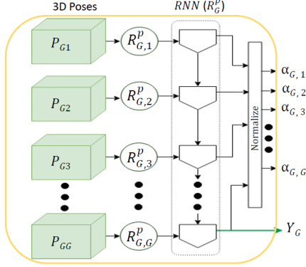
Figure 5. Temporal Segment attention ( TS - att ) from 3D poses for a given granularity G . P_{Gi} being input to the RNN R_{G,i}^p followed by their combination using RNN R_G^p to assign soft-weights \alpha_{G,j} .
