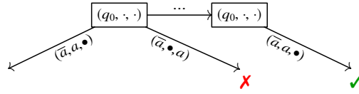
Fig. 3. Fragment of a possible service composition
