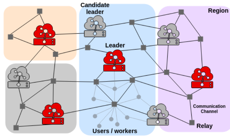
Fig. 1. SCR from a structural perspective—see description in Section 3.1. Notation: “gateway-like” nodes denote candidate leaders (red for active ones, grey for unelected ones); small grey squares denote relays; small grey circles denote users/workers.
