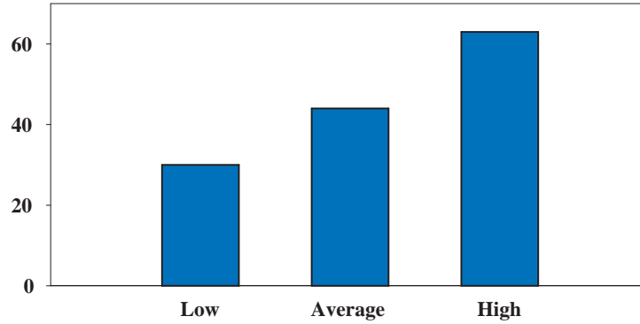
Fig. 1. Class distribution
