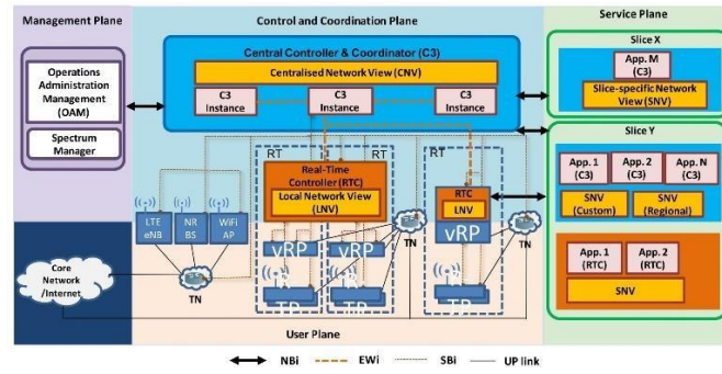
Fig. 1. COHERENT Architecture [8].
