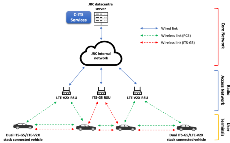
Fig. 6. The ITS-G5/LTE-V2X Testbed at JRC Ispra, in Italy.
