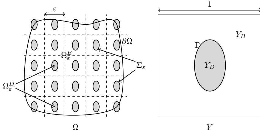
FIGURE 1. On the left: the idealised full 2D domain, \Omega . On the right: the periodic cell, Y .
