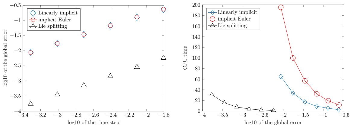
FIGURE 3. Comparison of methods of order 1 applied to (3.2): On the left hand side, maximal numerical error as a function of the time step (logarithmic scales); on the right hand side, CPU time (in seconds) as a function of the maximal numerical error.
