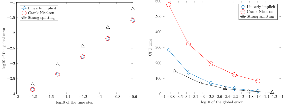
FIGURE 4. Comparison of methods of order 2 applied to (3.2): On the left hand side, maximal numerical error as a function of the time step (logarithmic scales); on the right hand side, CPU time (in seconds) as a function of the maximal numerical error.
