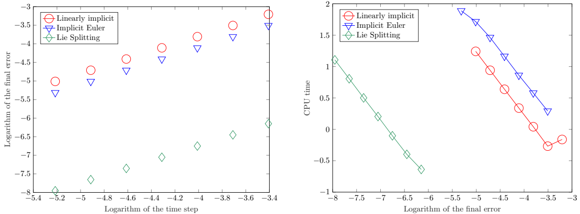
FIGURE 8. Comparison of methods of order 1 applied to (3.10): On the left hand side, maximal numerical error as a function of the time step (logarithmic scales); on the right hand side, CPU time (in seconds) as a function of the maximal numerical error.
