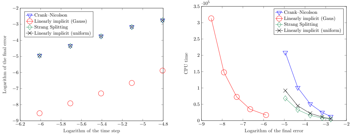
FIGURE 7. Comparison of methods of order 2 applied to (3.7): On the left hand side, maximal numerical error as a function of the time step (logarithmic scales); on the right hand side, CPU time (in seconds) as a function of the maximal numerical error.
