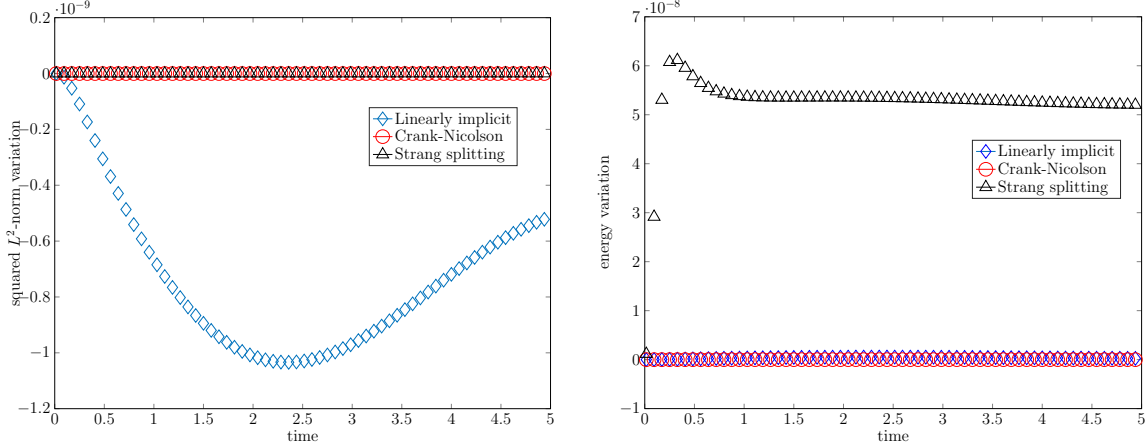
FIGURE 5. Comparison of methods of order 2 for mass and energy conservations: On the left hand side, variation of the mass with respect to time; on the right hand side, variation of the energy with respect to time
