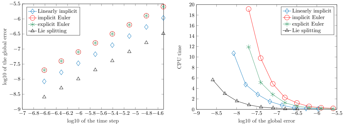
FIGURE 1. Comparison of methods of order 1 applied to (3.1): On the left hand side, maximal numerical error as a function of the time step (logarithmic scales); on the right hand side, CPU time (in seconds) as a function of the maximal numerical error.
