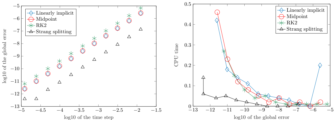
FIGURE 2. Comparison of methods of order 2 applied to (3.1): On the left hand side, maximal numerical error as a function of the time step (logarithmic scales); on the right hand side, CPU time (in seconds) as a function of the maximal numerical error.
