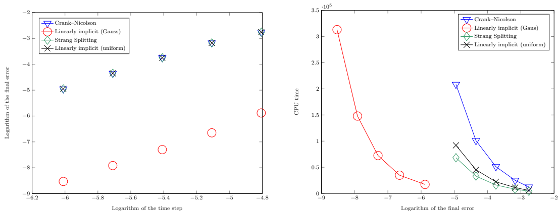
Fig. 6 Comparison of methods of order 2 applied to (45): On the left hand side, maximal numerical error as a function of the time step (logarithmic scales); on the right hand side, CPU time (in seconds) as a function of the maximal numerical error.
