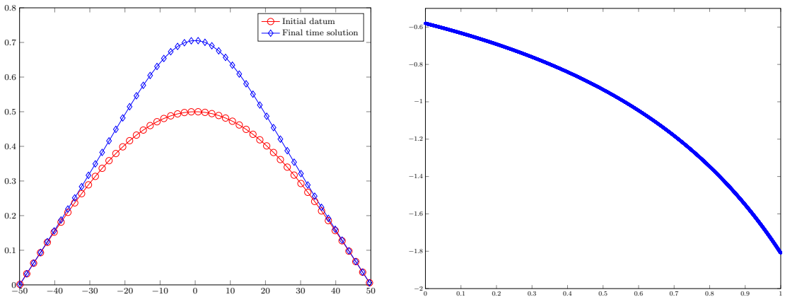
Fig. 8 Initial datum and solution at the final time T = 1 with respect to space (left hand side) and evolution of E_{rLx} with respect to time (right hand side).
