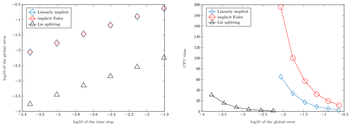
Fig. 3 Comparison of methods of order 1 applied to (40): On the left hand side, maximal numerical error as a function of the time step (logarithmic scales); on the right hand side, CPU time (in seconds) as a function of the maximal numerical error.
