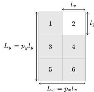
Fig. 5 2D domain used in the simulation of the nonlinear Schrödinger equation (45)
