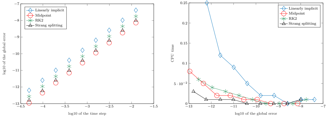
Fig. 2 Comparison of methods of order 2 applied to (39): On the left hand side, maximal numerical error as a function of the time step (logarithmic scales); on the right hand side, CPU time (in seconds) as a function of the maximal numerical error.
