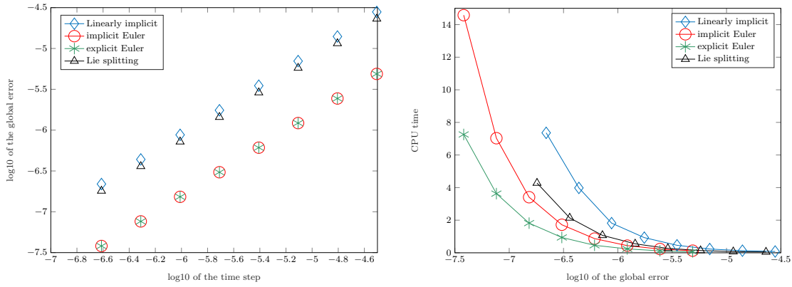
Fig. 1 Comparison of methods of order 1 applied to (39): On the left hand side, maximal numerical error as a function of the time step (logarithmic scales); on the right hand side, CPU time (in seconds) as a function of the maximal numerical error.
