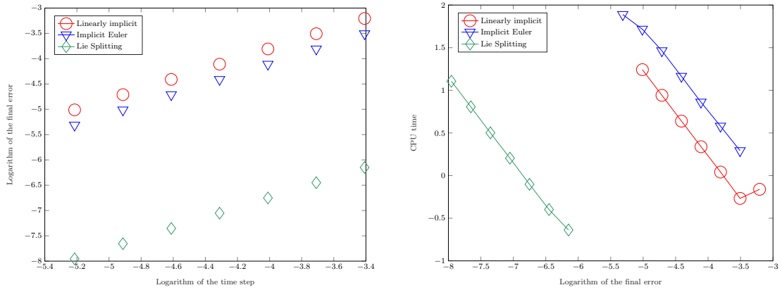
Fig. 7 Comparison of methods of order 1 applied to (47): On the left hand side, maximal numerical error as a function of the time step (logarithmic scales); on the right hand side, CPU time (in seconds) as a function of the maximal numerical error.
