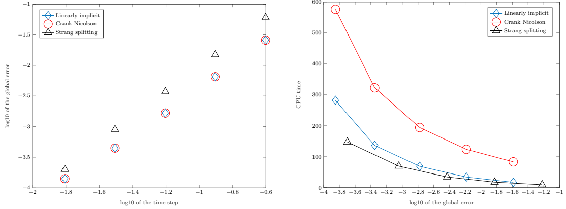
Fig. 4 Comparison of methods of order 2 applied to (40): On the left hand side, maximal numerical error as a function of the time step (logarithmic scales); on the right hand side, CPU time (in seconds) as a function of the maximal numerical error.
