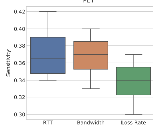
Fig. 9: PLT sensitivity to Net QoS
