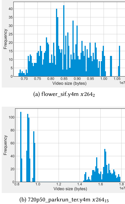
Fig. 2. The size distribution of 1,152 configurations of x264 over two input videos
