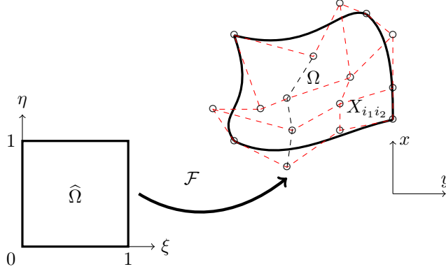
Figure 1: NURBS representation
