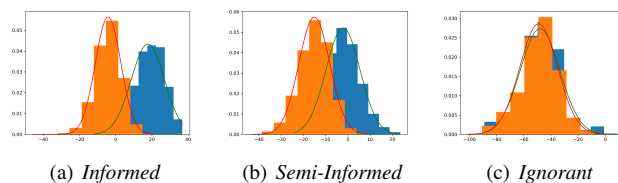
Fig. 1. I-vector score distribution for trials conducted on VTLN (strategy random ) converted data by Informed , Semi-Informed , or Ignorant attackers. The orange distribution indicates impostor scores, while the blue distribution indicates genuine scores. The crossing between the two curves indicates the threshold for EER. More overlap means greater confusion, hence greater privacy protection.
