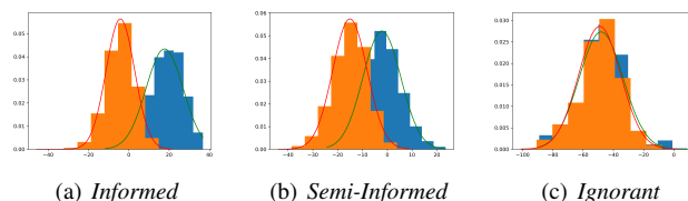
Fig. 1. I-vector score distribution for trials conducted on VTLN (strategy random ) converted data by Informed , Semi-Informed , or Ignorant attackers. The orange distribution indicates impostor scores, while the blue distribution indicates genuine scores. The crossing between the two curves indicates the threshold for EER. More overlap means greater confusion, hence greater privacy protection.
