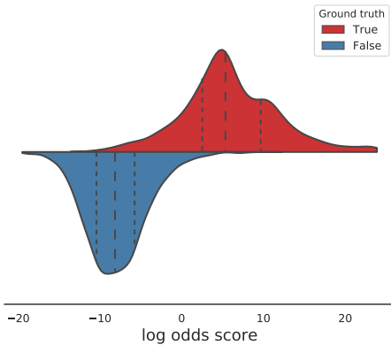
(a) Identification probabilistic scores output by BayesPairing2 for 4500 true hits and 4500 false hits
