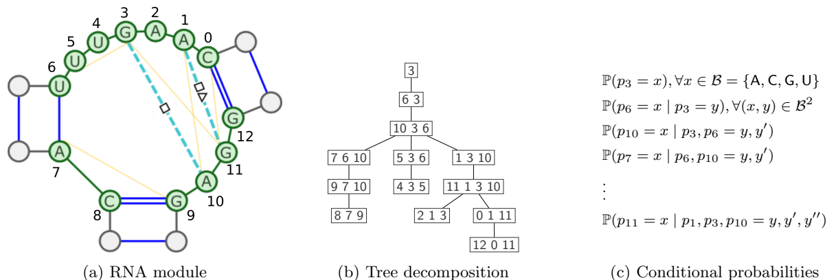
Fig. 2: An RNA 3D module (2a), here the three-way junction of the TPP riboswitch, represented in green, drawn in its structural context. Dashed and dotted lines respectively represent non-canonical base pairs and stacking interactions. A tree decomposition (2b) of the module represents the dependencies between the module positions, leading to conditional probabilities (2c), estimated from available sequence data
