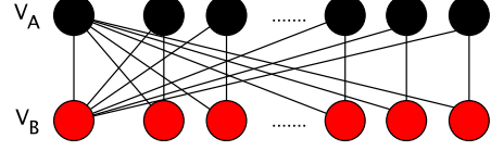
Figure 1: A toy bipartite graph G = (V_A \cup V_B, E) with vertex sets V_A and V_B . Except for the leftmost vertices from each vertex set, each vertex has two neighbors and will be removed by Rule-2 of KS. For every G^{(t)} , the merged vertices will have degrees (n+1-t) and 2. Hence, the total time for the naive KS implementation on this instance is \Theta(n^2) .
