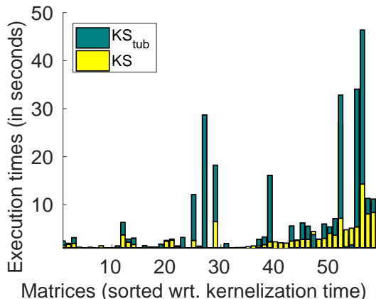
(b) Overall time comparison between KS and \text{KS}_{\text{TUB}} .
