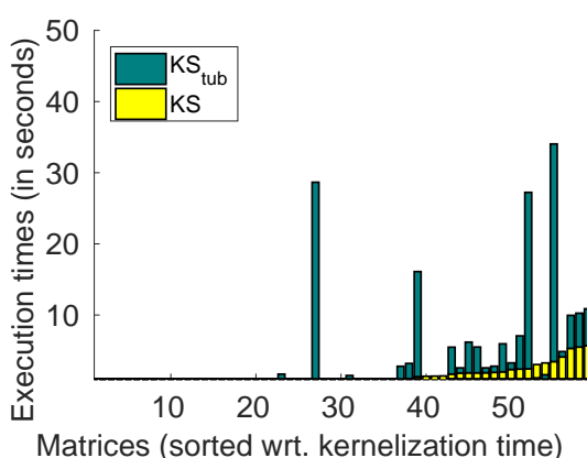
(a) Comparison only for kernelization between KS and \text{KS}_{\text{TUB}} .
