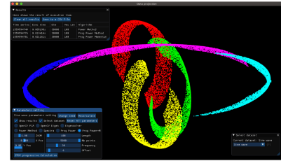
(c) PPCA: Progressive PCA for Massive Time-Series
