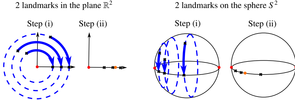
Figure 9.2 Steps (i)-(ii) of template estimation. The 3 black plus signs in \mathbb{R}^2 (left) or \mathbb{S}^2 (right) represent the 3 data. The 3 dotted blue curves are their orbits. In Step (i), the data are registered. The 3 black crosses in \mathbb{R}_+ (positive x-axis) (left) or [0, \pi] (right) represent the registered data. In Step (ii), the Fréchet mean of the registered data is computed and shown in orange.
