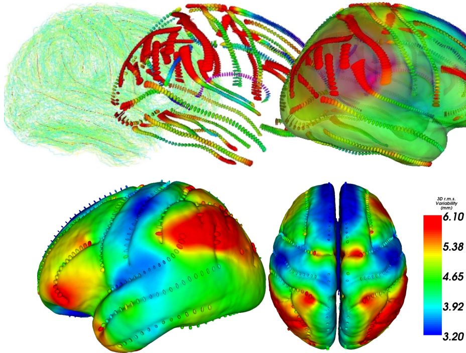
Figure 3.9 Top: From sulcal lines to the brain variability. Left : sulcal lines of 80 subjects in green with the mean sulcal lines in red. Middle: variability measured along the mean sulcal lines (covariance matrix at one sigma). Right: the color encodes the amount of variability everywhere on the cortex after the extrapolation of the covariance onto the whole 3D space. Bottom: The 366 SPD matrices selected along each sulcal lines, and the trace of the extrapolated covariance matrix. Lateral view from the left (on the left) and from above (right). Images courtesy of P. Fillard.
