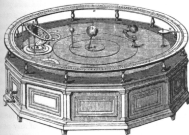
Ferguson's Orrery.
