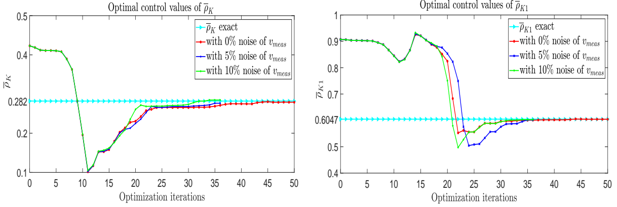
FIGURE 10. The evolution of the optimal control solution \bar{\rho}_K (left) and \bar{\rho}_{K1} (right) during the optimization iterations.
