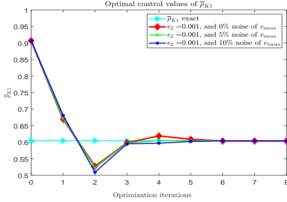
FIGURE 5. The evolution of the optimal control solution \bar{p}_{K1} during the optimization iterations.
