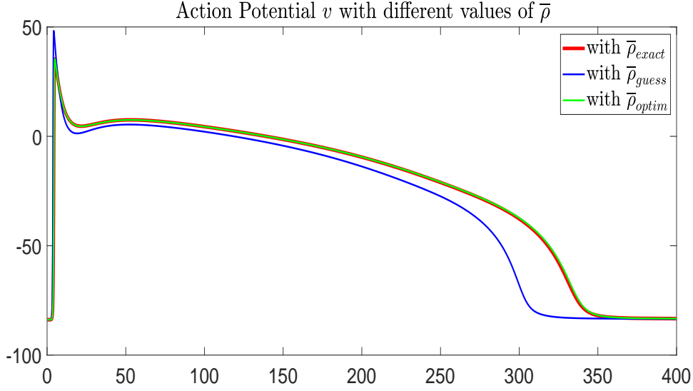
FIGURE 12. Action potential v with different value of \bar{\rho}
