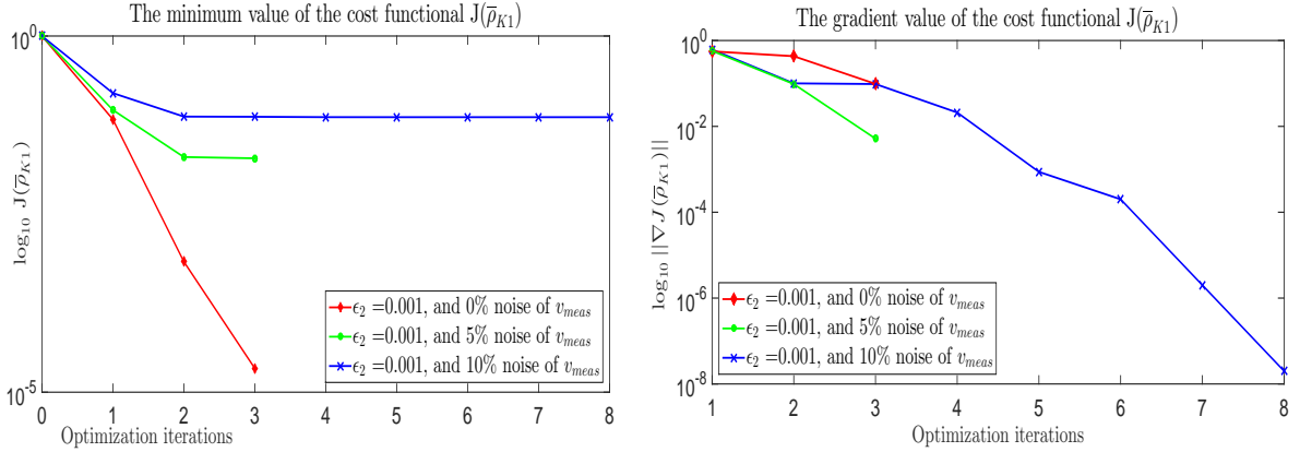
FIGURE 6. Left: Log scale plot of the cost function \mathcal{I}(\bar{p}_{K1}) . Right: Log scale plot of the norm of its gradient during the optimization procedure.
