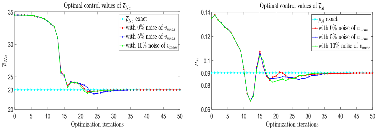
FIGURE 9. The evolution of the optimal control solution \bar{\varrho}_{Na} (left) and \bar{\varrho}_{si} (right) during the optimization iterations.
