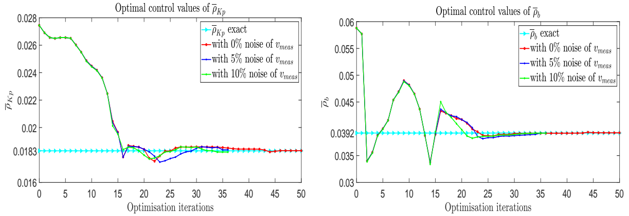
FIGURE 11. The evolution of the optimal control solution \bar{\rho}_{Kp} (left) and \bar{\rho}_b (right) during the optimization iterations.
