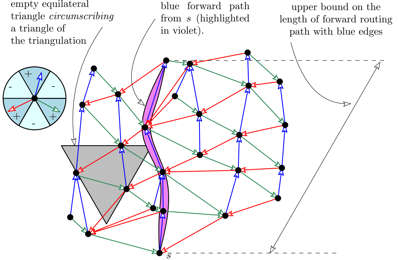
Figure 3: A TD -Delaunay triangulation (half- \Theta_6 -graph).
