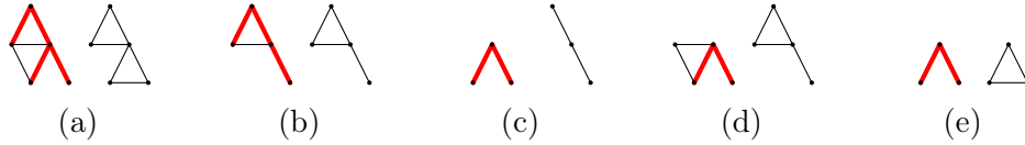
Figure 1: (a) Two graphs G and H , where T is shown in red; (b) a T -MCCIS that is also MCCIS; (c) a T -MCCIS; (d) not a T -MCCIS since it is a MCCIS but not spanned by T ; (e) not a T -MCCIS since it is spanned by T but is not a common induced subgraph.
