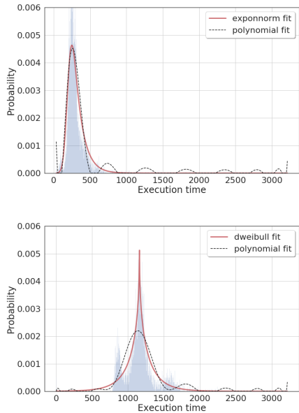
Fig. 1. Performance behavior for two stochastic functions together with two transformations into the continuous domain (top: Functional QA and pre-processing application, bottom: Deep brain structure segmentation application). Runs done during 2017 by the neuroscience department at the Vanderbilt University.
