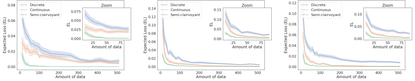
Fig. 4. Results for the truncated normal distributions (left: low variance, middle: high variance) and the truncated exponential distribution (right)
